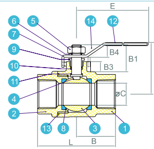
■ FIG. 20-30 REDUCED PORT 1/4" TO 1" 2000 PSI 1 1/4" TO 2" 1500 PSI
