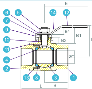
■ FIG. 20-40 FULL PORT 1/4" TO 1" 2000 PSI 1 1/4" TO 2" 1500 PSI
